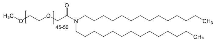
Figure 2 ALC-0159 structure
